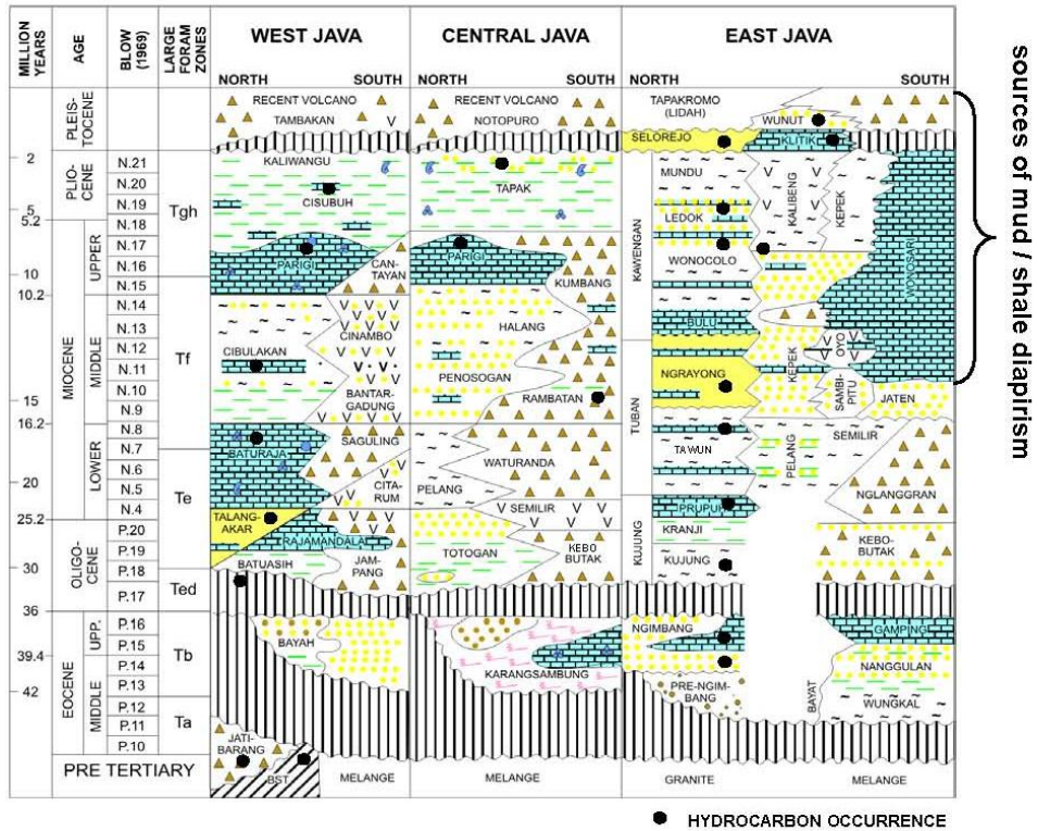
Figure 9 – Stratigraphy of West Java, Central Java, and East Java showing the occurrences of hydrocarbons
